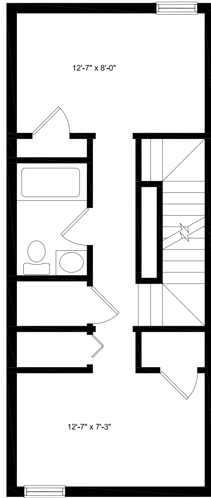
SECOND FLOOR
