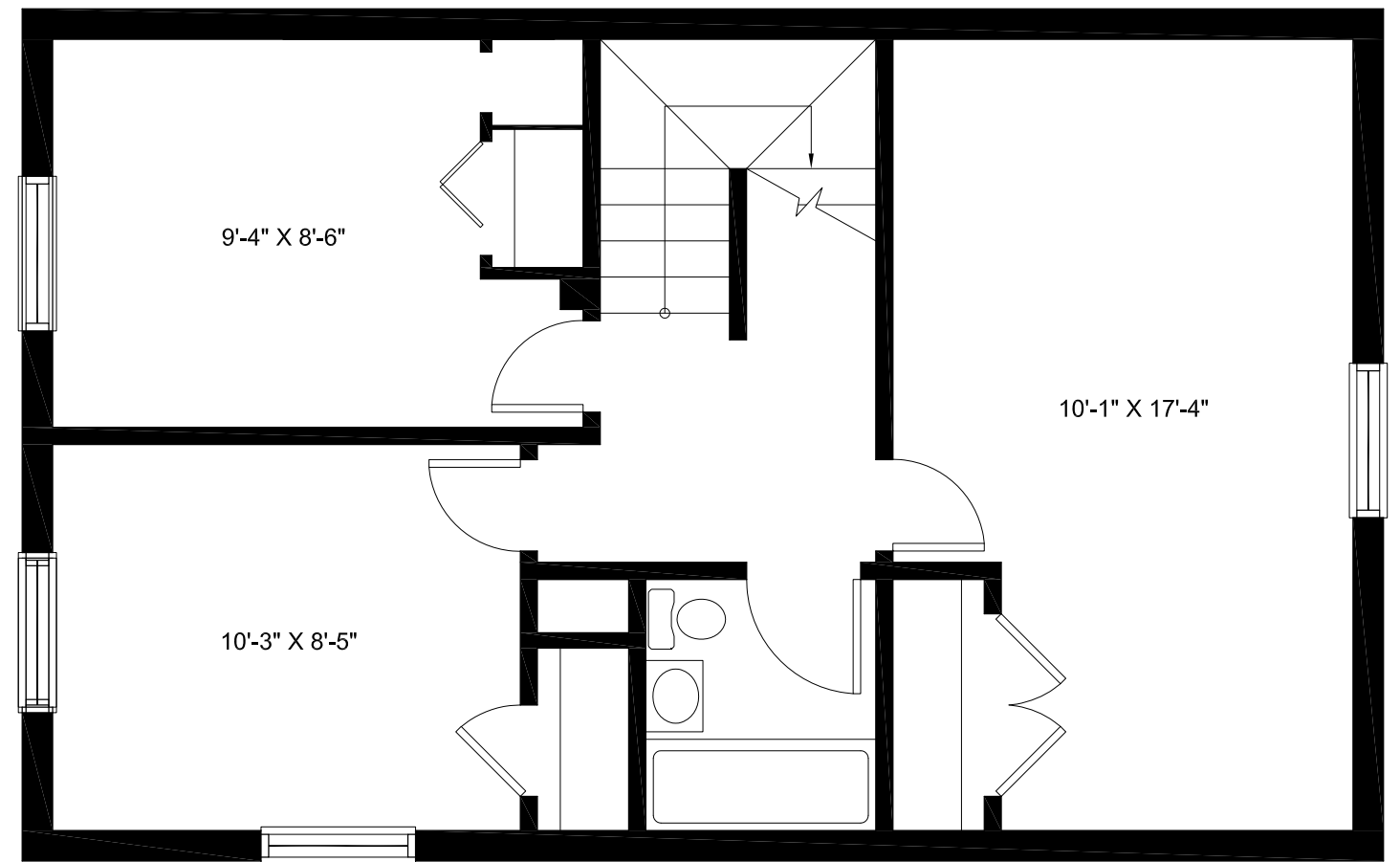
SECOND FLOOR
